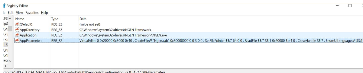
Figure 27 // srvany-ng is configured to execute the winapiexec tool with InvisiMole's shellcode
