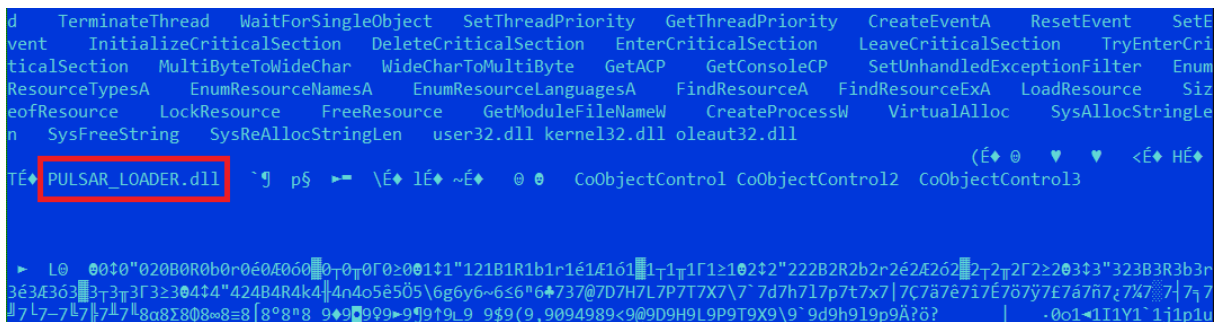
Figure 14 // InvisiMole's component with internal name PULSAR_LOADER.dll
