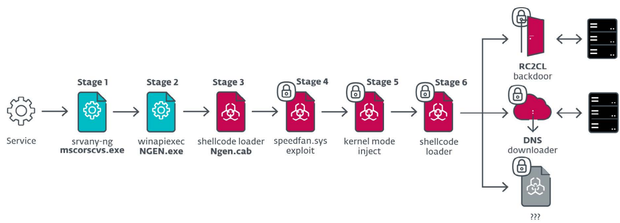
Figure 25 // Execution chain exploiting vulnerability in the speedfan.sys driver
