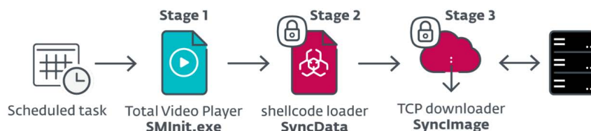
Figure 22 // InvisiMole's SMInit exploit chain
