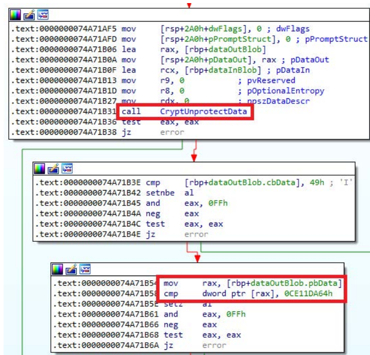
Figure 2 // InvisiMole's loader uses CryptUnprotectData API to decrypt the next stage, and then checks the decrypted blob for InvisiMole magic value 64 DA 11 CE
