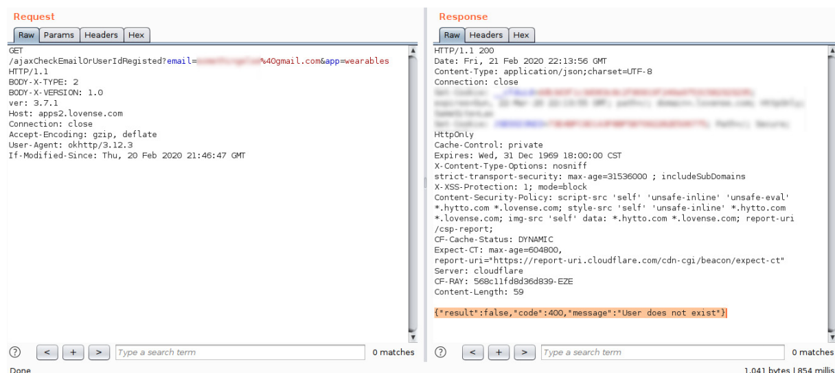
Figure 12// In contrast to Figure 11, here the server returns a negative response to a query about an email address
