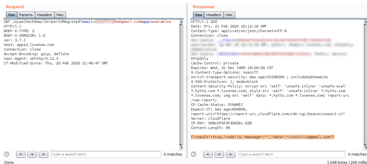
Figure 11// This GET request queries whether the supplied email address matches a user account on the Lovense platform. In this case, the result is successful.
